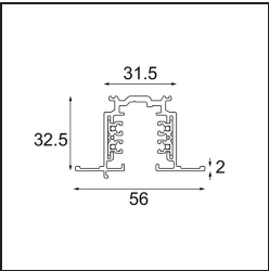
FFD_Track 230V Dali Profile Recessed 2000 White Shiny
