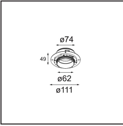
13515630 Concrete Ring 62 Standard Installation Housing
