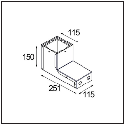
12349930 Installation Housing 115x115x150x251
