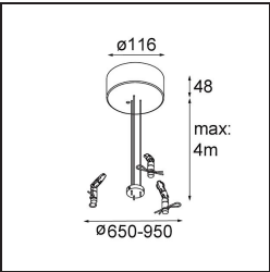
FFD_Flat moon suspension kit 4m / 3x0.75 triangle (3 cables) white struc
